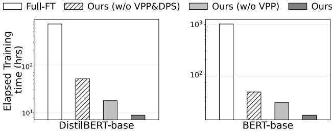
Figure 16: Model convergence delay with or without FwdLLM’s key designs, showing their significance. VPP means Variance-controlled Perturbation Pacing, and DPS means Discriminative Perturbation Sampling.
