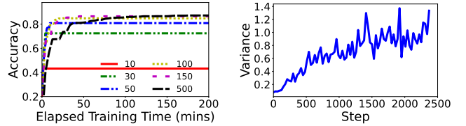
Figure 7: Optimal Global-PS varies across training.
