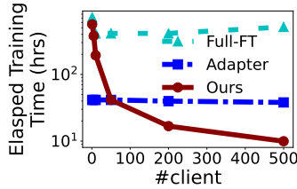
Figure 12: FwdLLM performance with different #clients.
