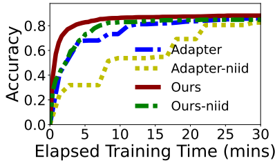
Figure 13: Non-iid performance for AGNEWS on DistilBERT.
