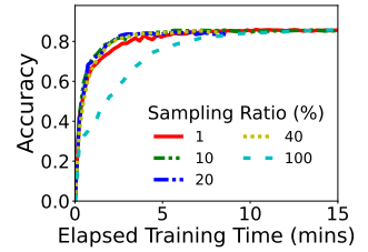
Figure 18: Different sampling ratio. Model:BERT. Dataset:AGNews
