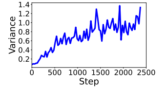
Figure 7: Optimal Global-PS varies across training.
